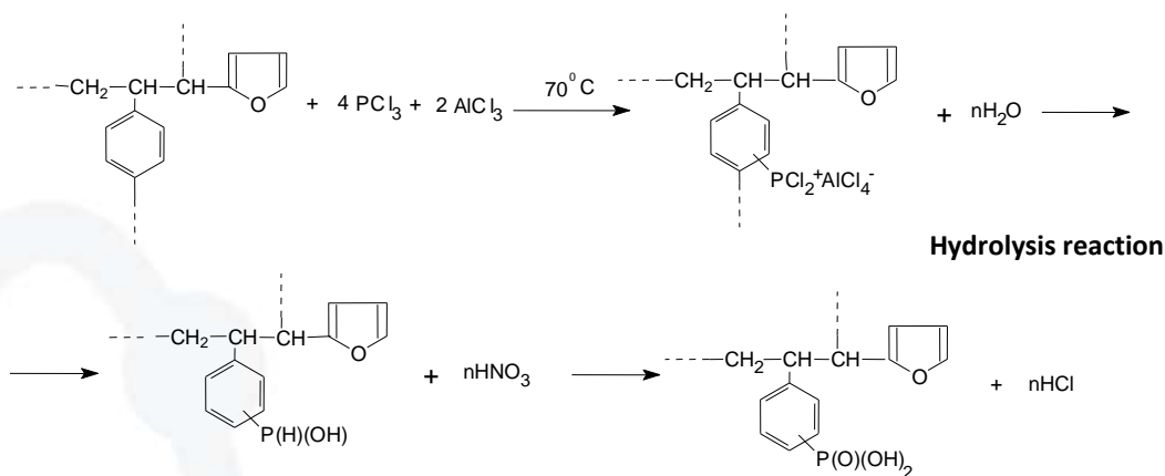
Reaction of the oxidation of the cation exchanger with nitric acid
