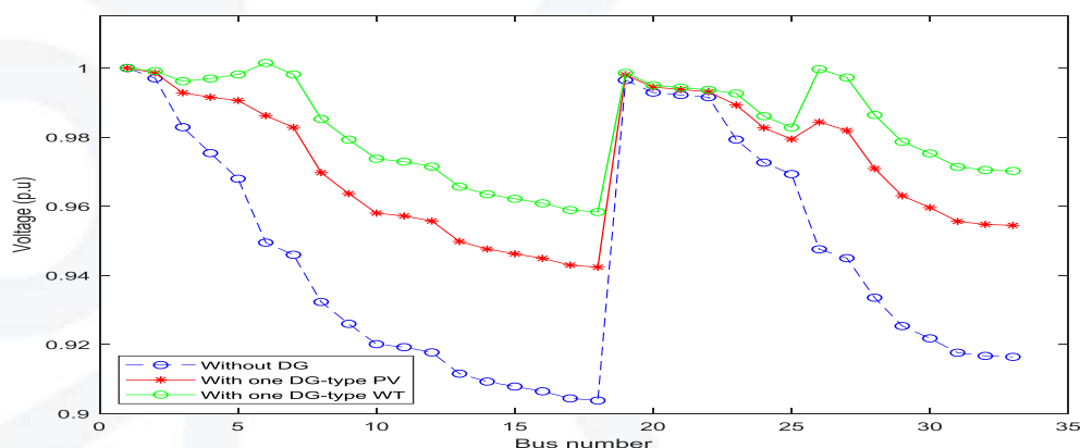
Fig. 4. Impact of two DG units on the voltage profile.
