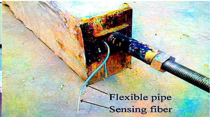
Figure 7. Photograph of a Beam Strengthened with FRP Cable
