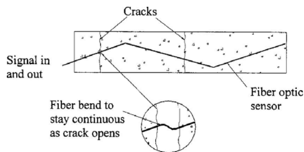
Figure 5. Principle of Operation of the Zigzag Sensor
