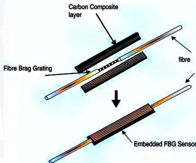
Figure 3. Strain Sensor Placed Between Layers of Composite Material.
