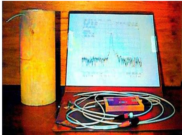
Fig. 9. A Concrete Cylinder with an Embedment of FBG Sensor (left) Connection to Cable and Terminal (right)
