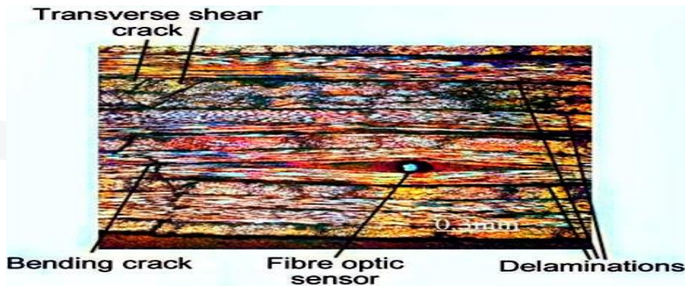
Figure 8. Section through Damaged Area of FRP Containing Fiber Optic
