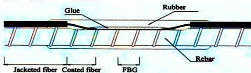
Figure 4. Scheme of the Strain Sensor
