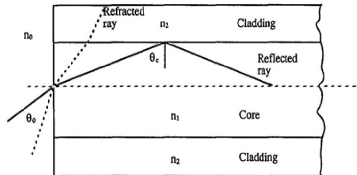
Figure 2. Basic Geometry of Optical Fiber Sensor
