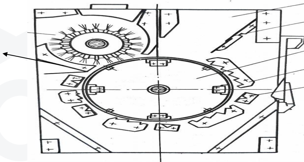
1-Figure.1-supply line, 2- router, 3-saw drum, 4- kolosnik cage , 5- router, 6-brush drum
