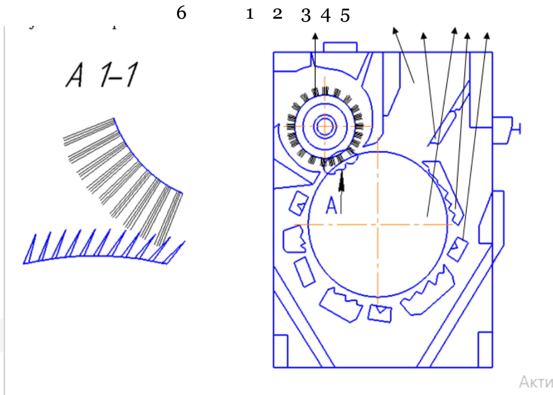
2-Figure. 1-Supply pipe , 2- guide , 3-needle, 4-column grate, 5-guide, 6- brush brush
