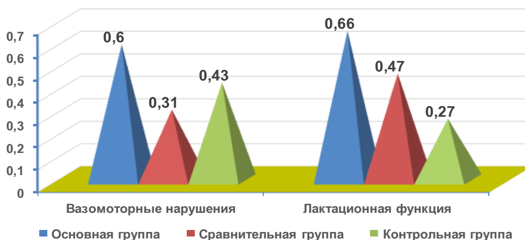
Fig. 2. indicators of the scale of lactation function and vasomotor disorders
