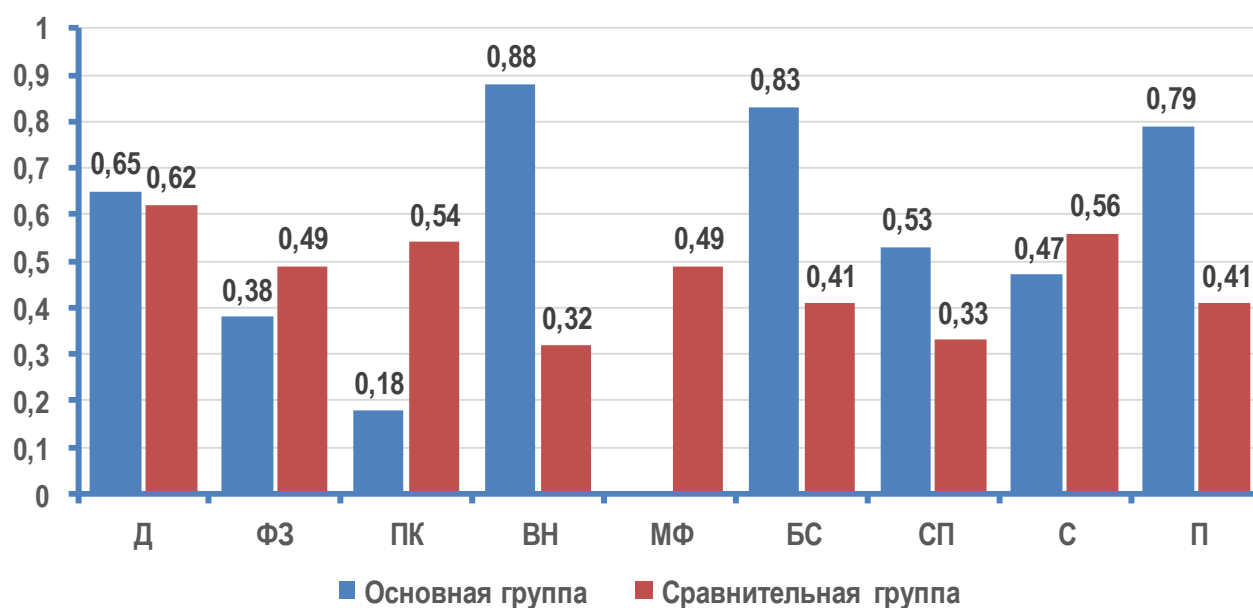
Fig. 1. Comparative characteristics of the average quality of life of women of fertile age with organ removal and women without organ removal with bleeding in the long term according to the questionnaire scales.
